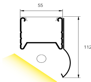
reflector lateral curvo
